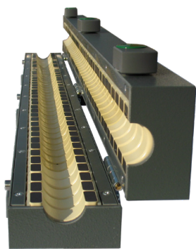
KEMA 801B, side view
